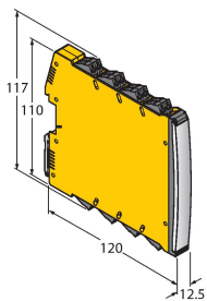
IMX12-DO01-2U-2U-0/24VDC 7580105
