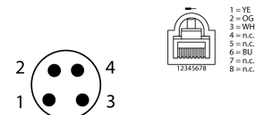
Circuit Diagram
