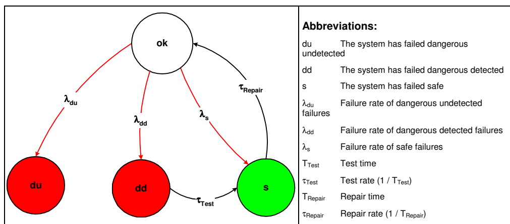
Figure 3: Markov model for a 1oo1D structure
