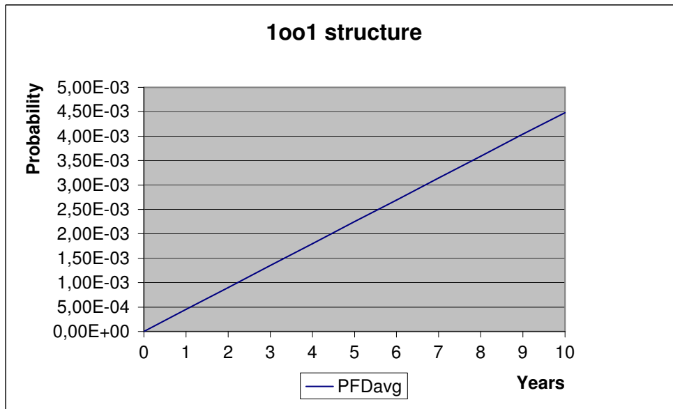
Figure 6: PFD_{Avg}(t)
