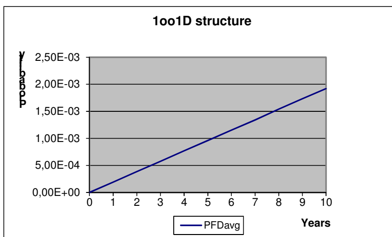
Figure 5: PFD AVG (t)
