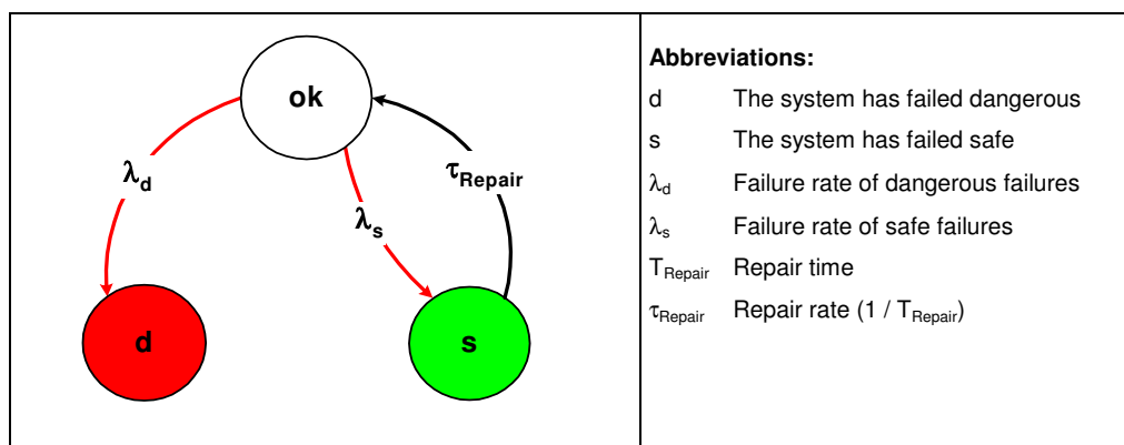
Figure 4: Markov model for a 1oo1 structure
