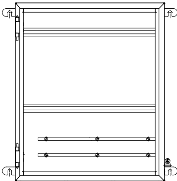
MOUNTING VIEW
