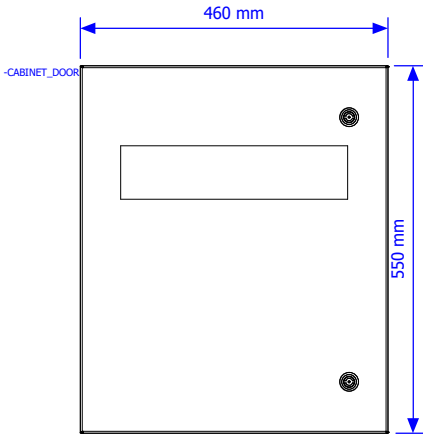
DOOR VIEW
