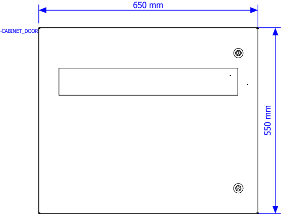
DOOR VIEW
