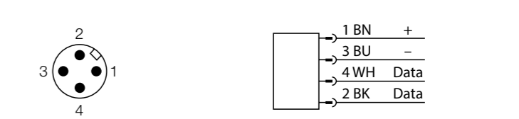
Connectors .../S2500
