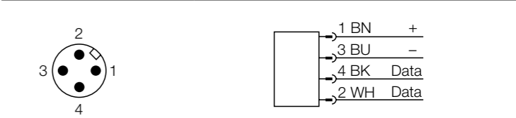
Connectors .../S2501
