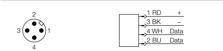
Connectors .../S2503
